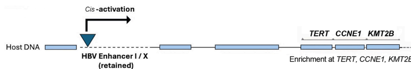
Fig. 2. Cis-activation mechanisms of HBV integration-mediated hepatocarcinogenesis. Retention of HBV enhancer I/X regulatory elements at integration sites promotes cis -regulatory activation of adjacent host genes. Clonal selection enriches integration events near oncogenic loci, including TERT , CCNE1 , and KMT2B , supporting their potential roles as functional drivers of hepatocarcinogenesis. CCNE1 , cyclin E1; HBV, hepatitis B virus; KMT2B , lysine methyltransferase 2B; TERT , telomerase reverse transcriptase.
